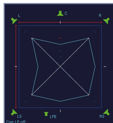
3 | Same as on the left but with the phase of the left channel rotated through 180^\circ . In the channel pairs L - R and L - LS each the correlation is r = -1 , there are no phantom sound sources locatable.
