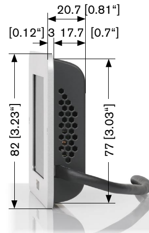
2 | Side view
