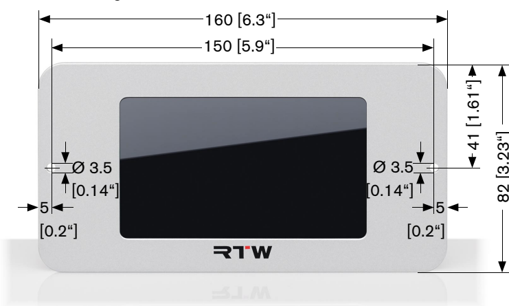
1 | Front view
