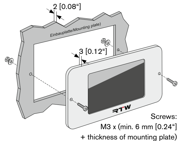
5 | Mounting
