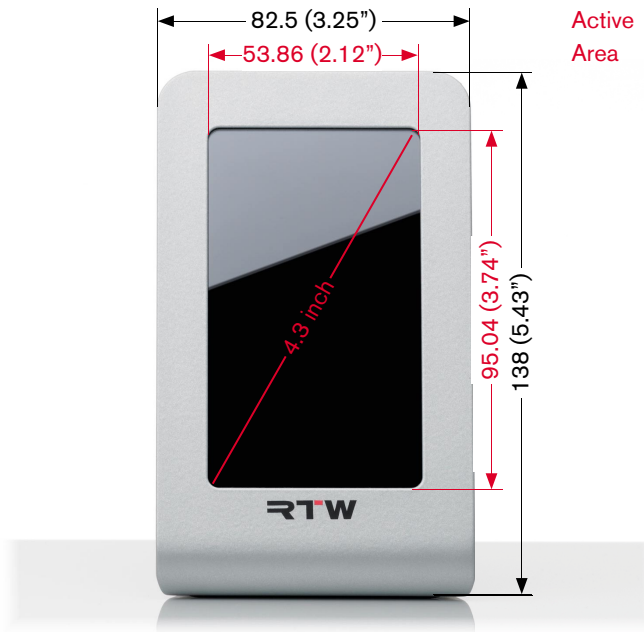
1 | Front view
