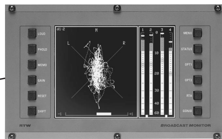
BroadcastMonitor 106nX-3U
