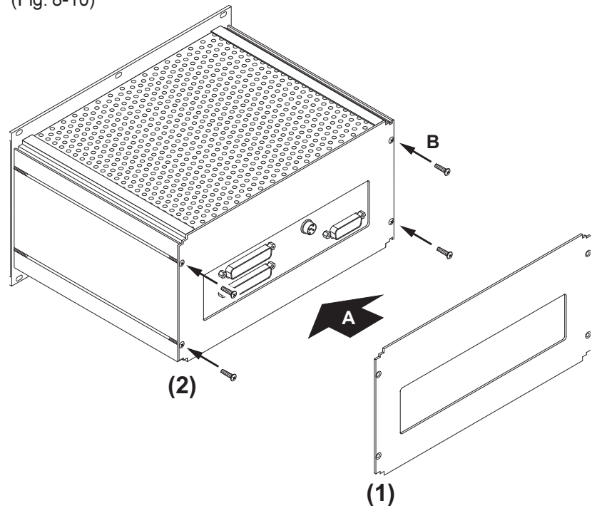
Fig. 8-10: Mounting the backplane cover
