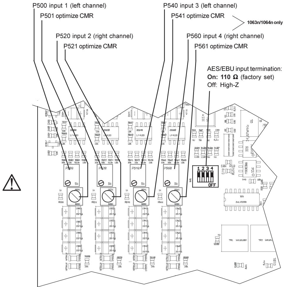
Fig. 8-1: Partial view of input pcb
